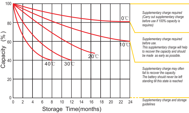
Storage Characteristics
