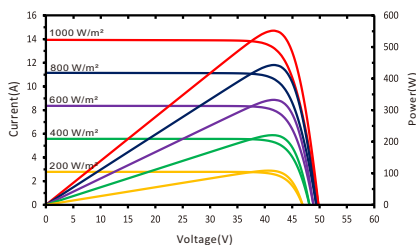
RSM144-9-550M I-V characteristics at different irradiances
